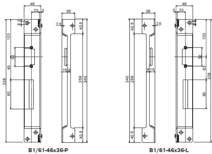
B1/61-46x36-P
