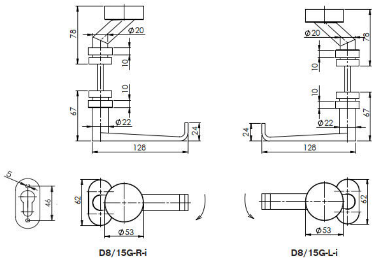
D8/15G-R-i
