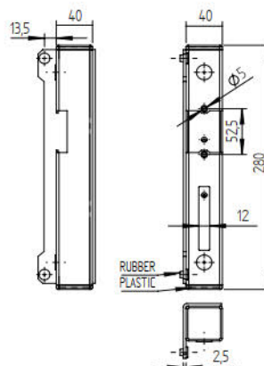
B1/61-46x36-P
